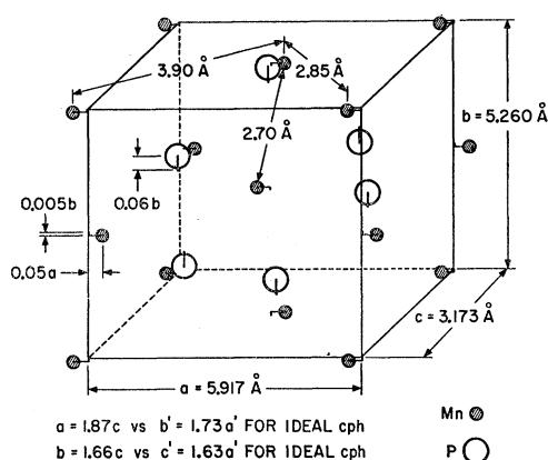
FIG. 1. The B31 structure of orthorhombic MnP.
