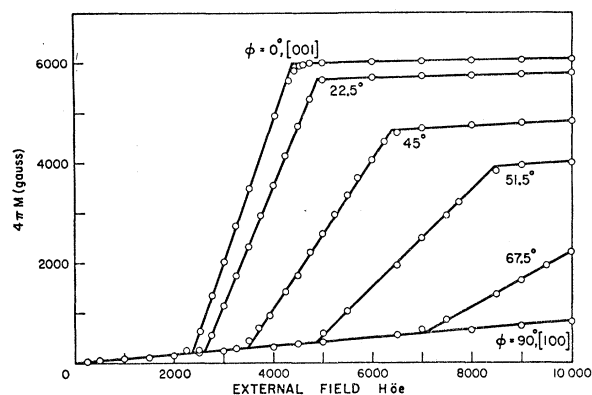
FIG. 12. Magnetization curves at 7.3°K in the ac plane. \varphi is the angle between H and the [001] direction and is 90° when H is along the [100] direction.
