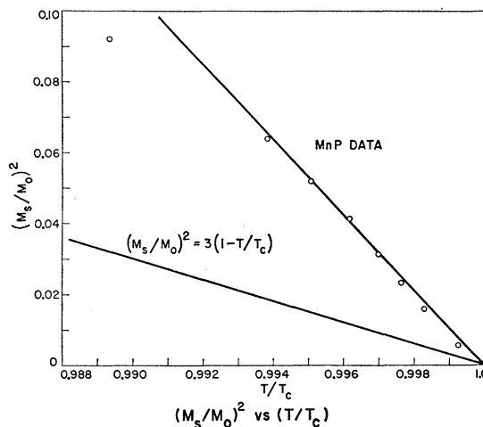
FIG. 4. (M_s/M_0)^2 versus (T/T_c) near the Curie point. The point at (M_s/M_0)^2 \approx 0.092 shows the beginning of the deviation from linearity.
