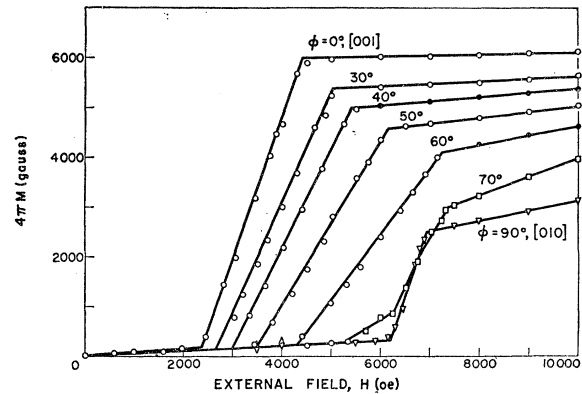
FIG. 11. Magnetization curves at 7.3°K in the bc plane. \varphi is the angle between H and the [001] direction and is 90° when H is along the [010] direction.
